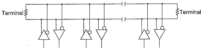
A bus structure is possible with the RS-485
